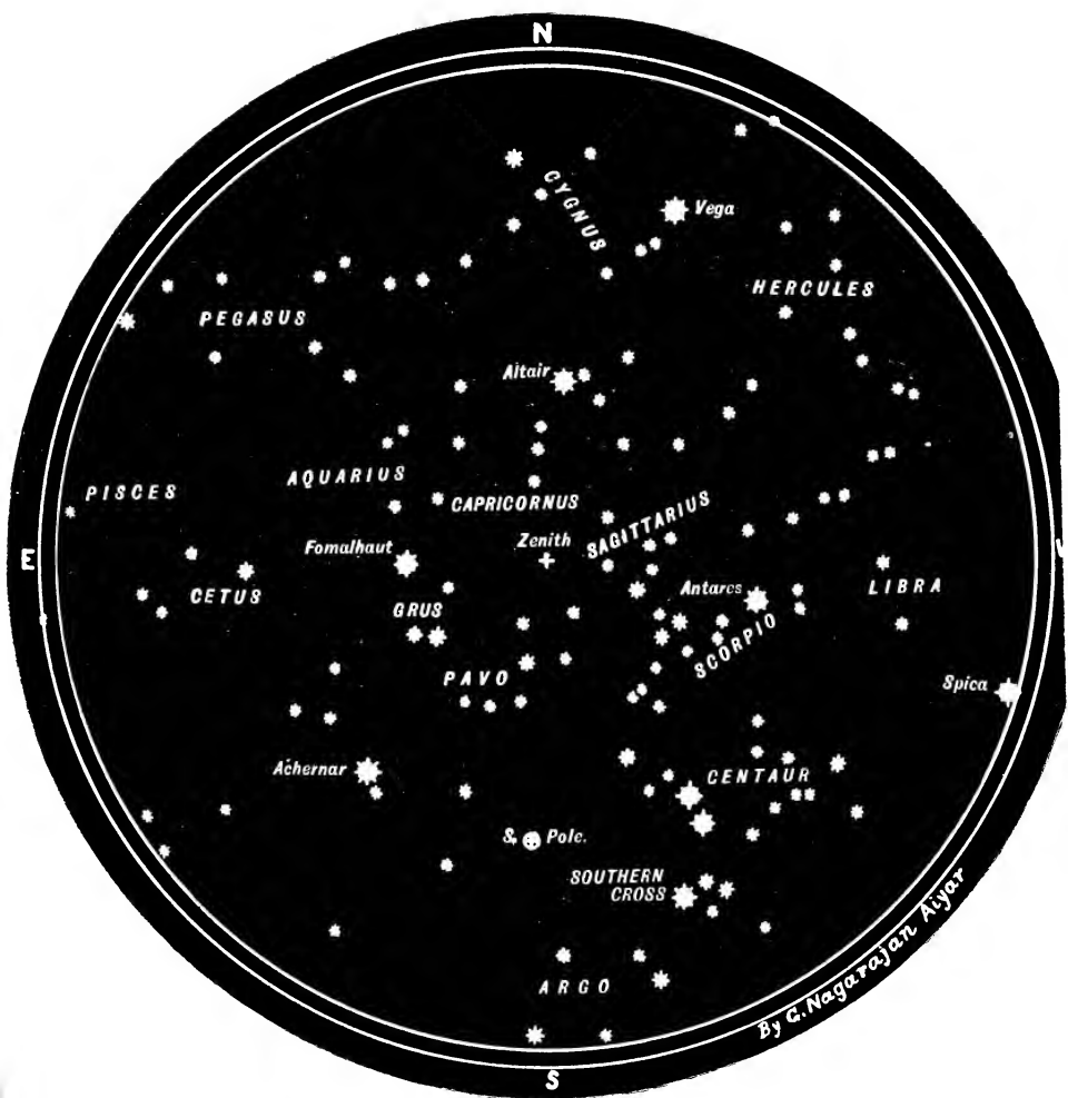
MAP OF STARS VISIBLE BEFORE DAWN IN PURGATORY. (17) (17)
